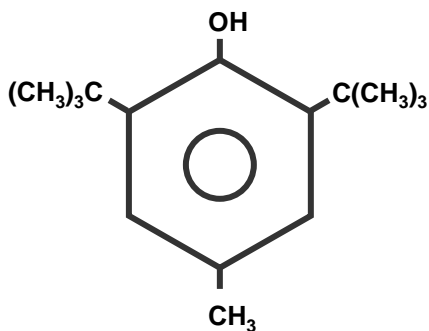
2,6-di-tert-butyl-p-cresol
